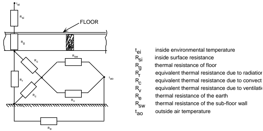
Figure 1: Thermal resistance network for heat flow through suspended floor
